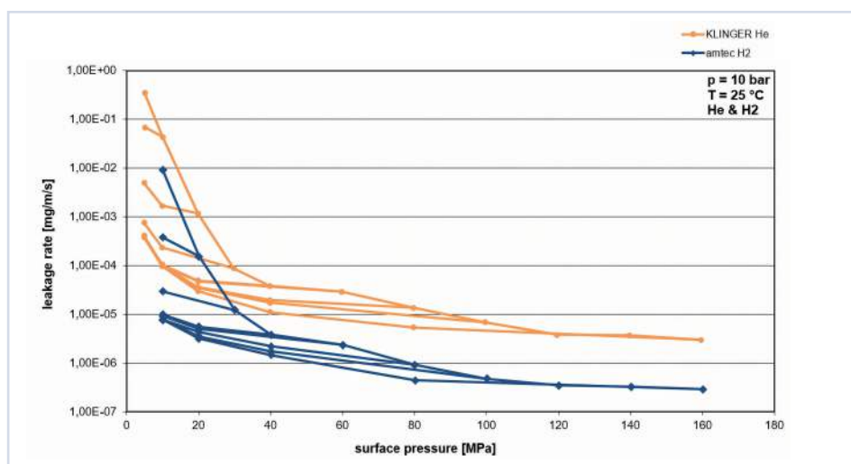
Graph #2: Leakage curves EN 13555 KLINGER top-chem 2003 92x49x2 mm
